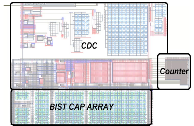
Fig. 8. Layout of the proposed CDC.
