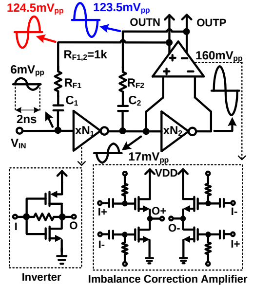
Fig. 3. The proposed wideband inverter-based single-to-differential (S-to-D) LNA. The voltage swing waveform at each node is shown when a 500 MHz RF signal with a power of -40 dBm is applied to the LNA.
