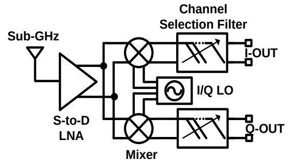
Fig. 1. Schematic of the proposed receiver front-end composed of wideband single-to-differential (S-to-D) low noise amplifier (LNA), in-phase/quadrature (I/Q) passive mixer and channel selection filter.
