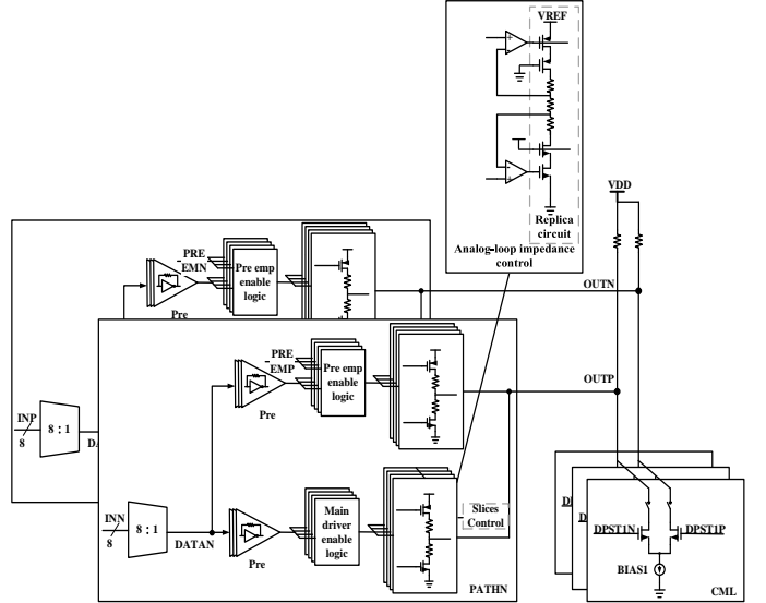
Fig. 4. Pre-emphasis logic with adjustable FIR top schematic.
