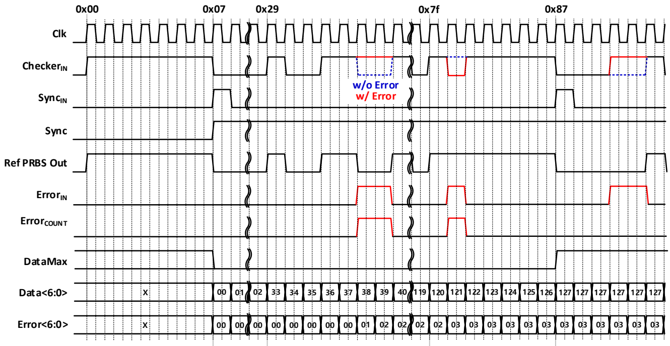
Fig. 7. PRBS checker operation.
