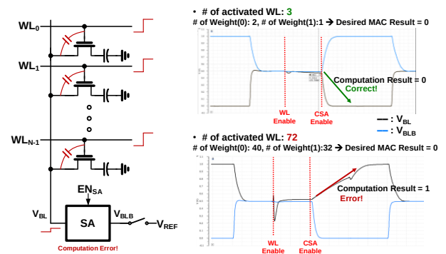
Fig. 4. Presence of Switching Non-ideality
