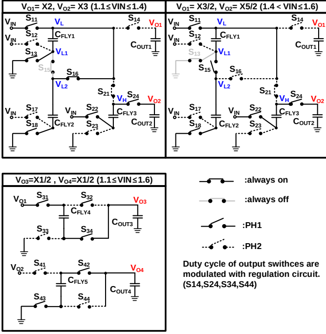
Fig. 2. Switch configuration of the proposed work. Bold lines and dashed lines represent PH1 and PH2, respectively.
