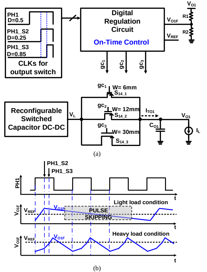
Fig. 3. Ordered-sequential switching configuration with feedback loop and output voltage at different load condition of V_{O1} ; (a) regulation circuit for V_{O1} , and (b) waveforms of V_{O1F} under various load conditions.
