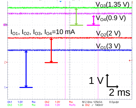
Fig. 7. Measured waveforms of the output voltages with ( V_{DD}=1.4 V).
