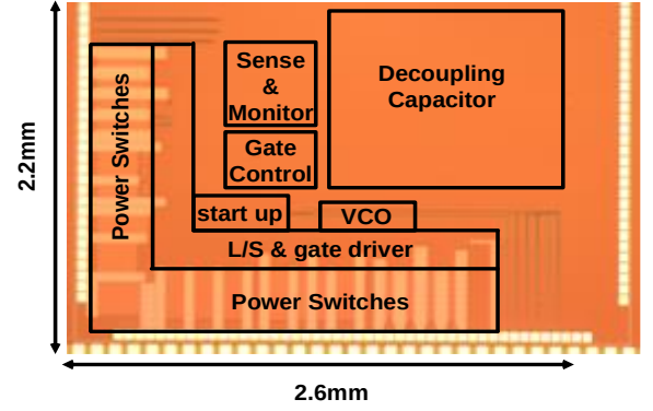
Fig. 6. Chip micrograph.
