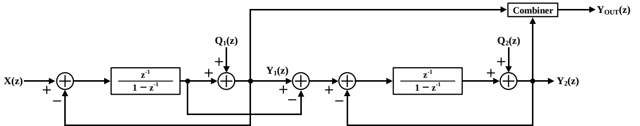
Fig. 1. Linear block model of MASH 1-1 DSM
