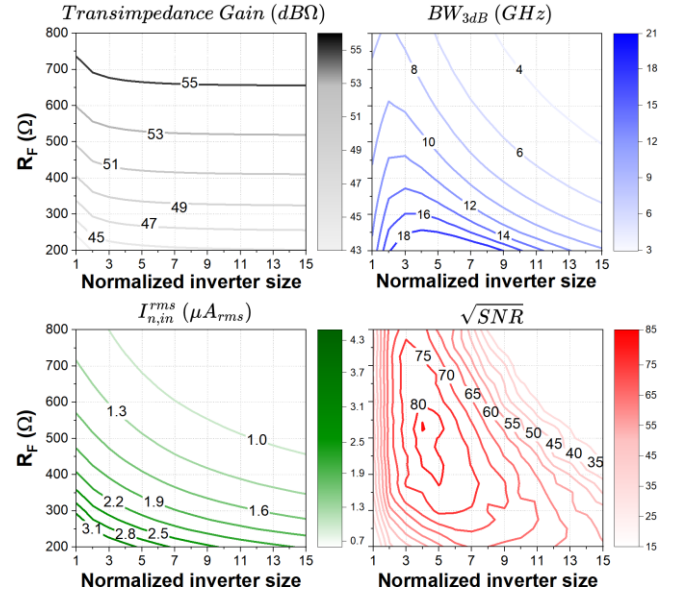
Fig. 3. the contour plot of the transimpedance gain, bandwidth, input-referred rms noise, and \sqrt{SNR} with respect to inverter size and R_F of SF-TIA ( C_{PAD} = 400 pF, L_b = 400 pH, C_L = 40 fF) using BAG.
