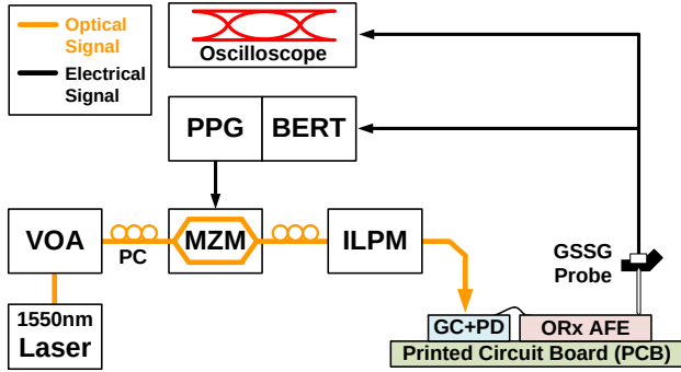
Fig. 8. Measurement setup.
