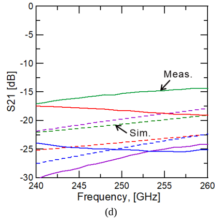
Fig. 4. (a) Layout and (b) photograph of the RTPS. (c) Differential phase and (d) insertion losses of the RTPS.
