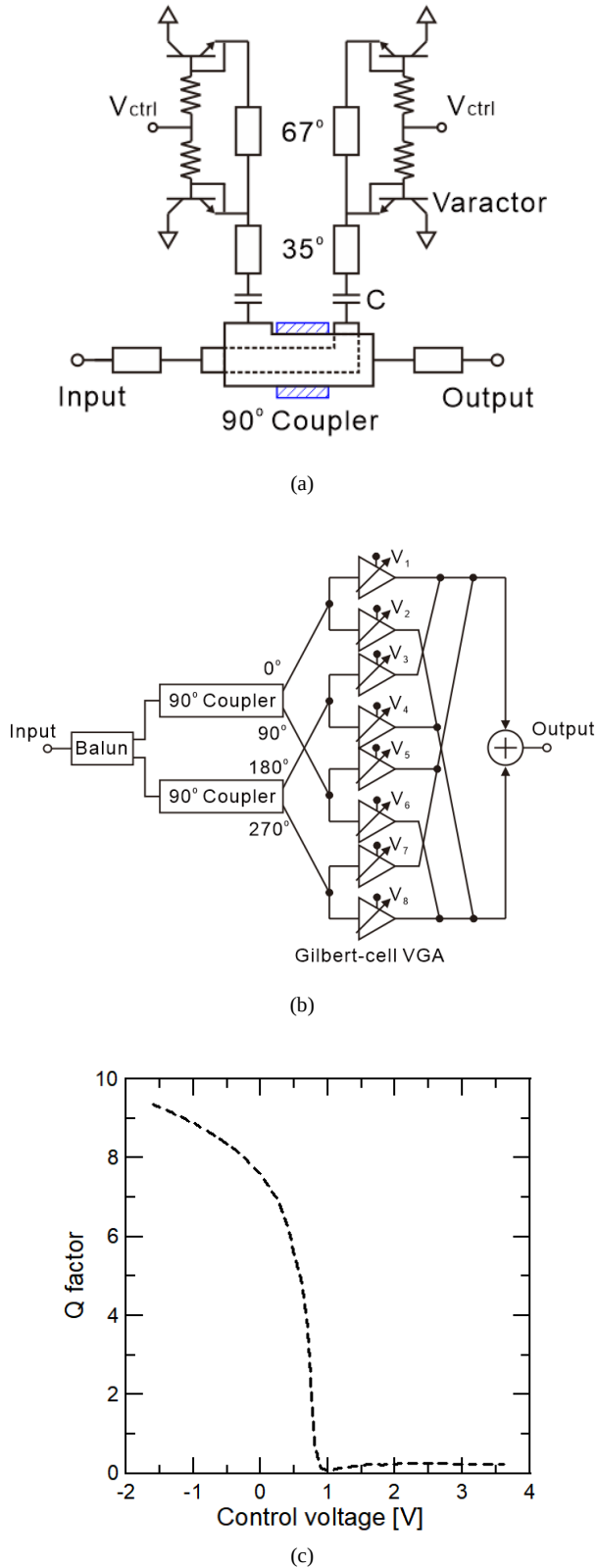
Fig. 3. (a) Schematic of fabricated RTPS unit cell, (b) block diagram of typical vector-sum phase shifter using Gilbert-cell VGAs and (c) Q-factor of diode-connected varactor.
