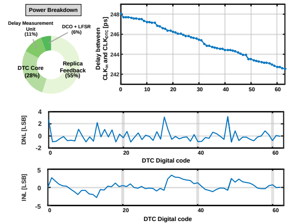
Fig. 7. Power breakdown and measured DTC linearity.
