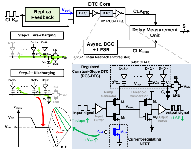
Fig. 1. Block diagram of core and architecture of the proposed DTC.
