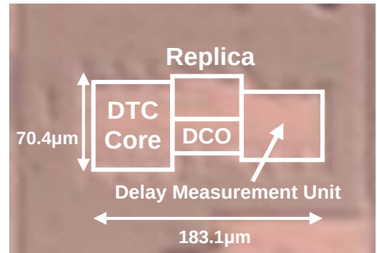
Fig. 6. Chip microphotograph.
