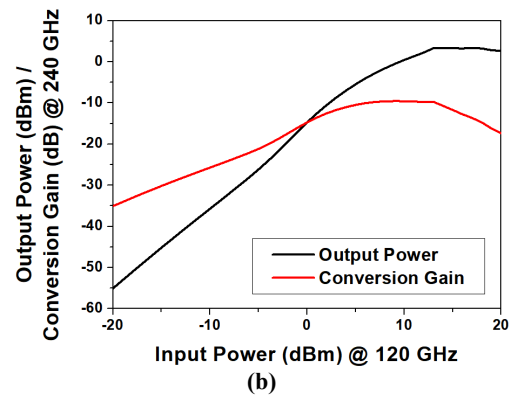
Fig. 5. Simulated output power against (a) output frequency and (b) input power and conversion gain at 120 GHz input frequency of the 240-GHz frequency doubler.
