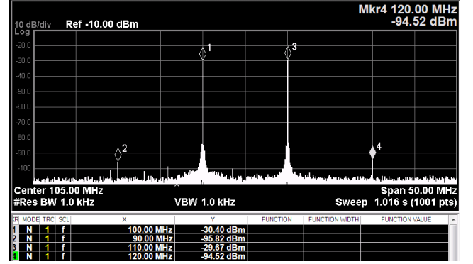
Fig. 6. Measured single-ended output spectrum of the proposed RF down-conversion mixer. RF Input power was set to -30 dBm and total loss by cables and probe tips is approximately 1.5 dB.
