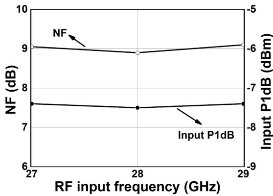
Fig. 9. Measured NF and input P1dB.
