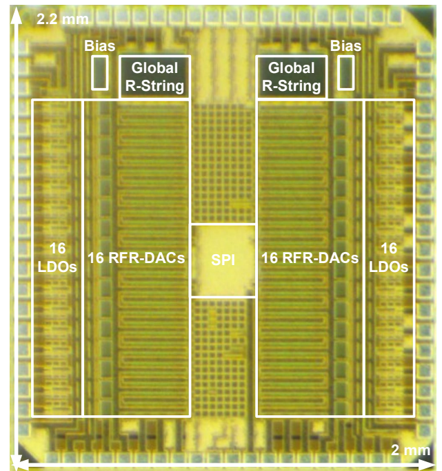
Fig. 13. Die micrograph of 0.18 \mu m CMOS test chip.
