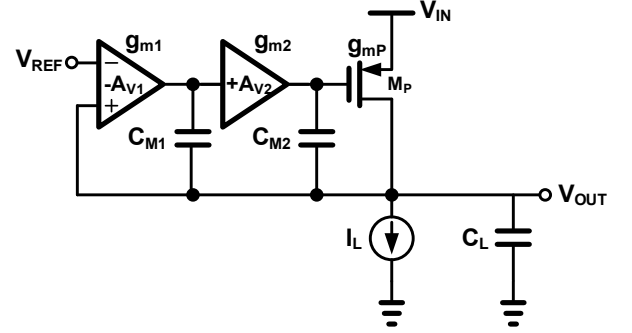
Fig. 7. 3-Stage LDO structure
