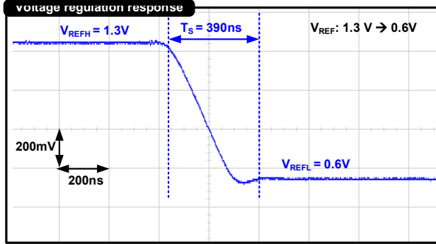
Fig. 9. Voltage regulation response with V_{REF} changing from = 1.3V to 0.6V.
