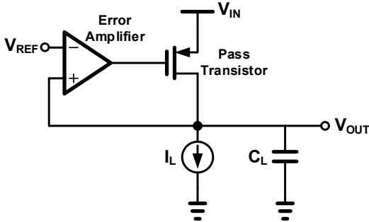
Fig. 3. Conventional low dropout regulator.
