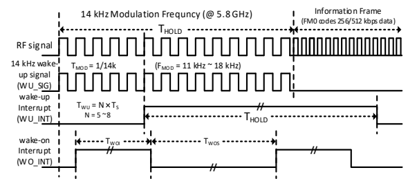
Fig. 6. RF wake-on and wake-up interrupt timing diagram
