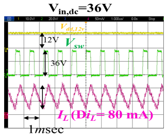
Fig. 14. Waveform of buck converter PMIC at operation of (a) V_{in,dc}=15\text{V} , and (b) V_{in,dc}=36\text{V} .
