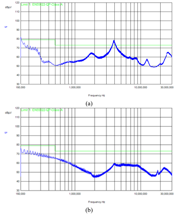
Fig. 17. Measured conducted emission of (a) 2-stage PEF and (b) 1-stage AEF with PMIC
