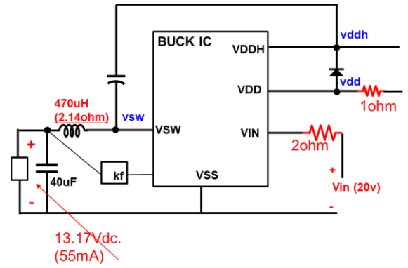
Fig. 13. Configuration of Test set-up
