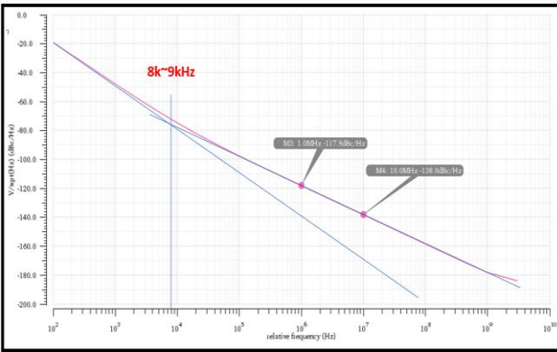
Fig. 10. Post layout phase noise simulation at 7.2GHz
