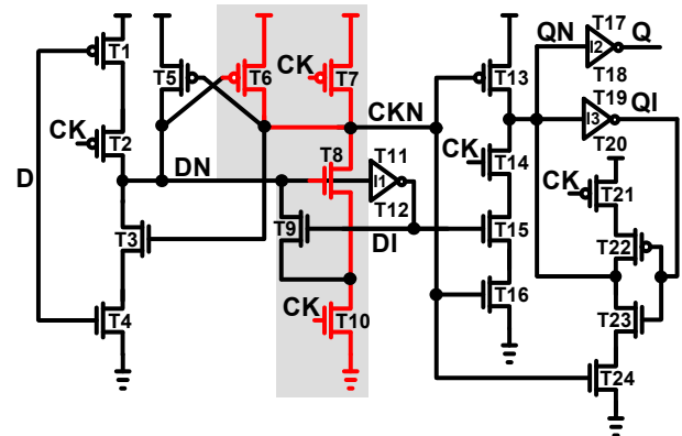
Fig. 2. Static single-phase contention-free flip-flop (S2CFF)
