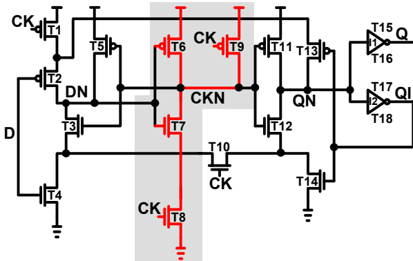
Fig. 4. 18-transistor single-phase clocked flip-flop (18TSPC)
