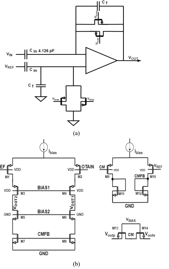
Fig. 3. (a) Top-level diagram of the capacitive-feedback amplifier. (b) The amplifier circuit
