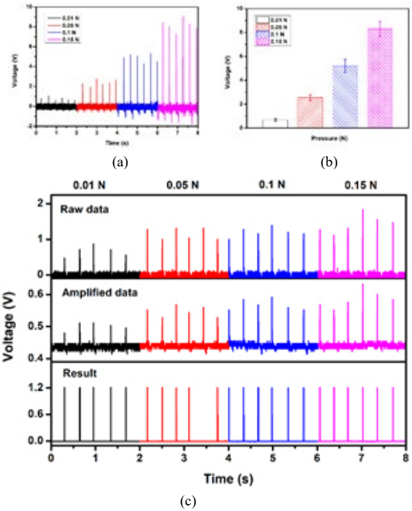
Fig. 9. (a) The output of the TENG device based on the tapping pressure. (b) The relationship between tapping pressure and the voltage output. (c) The detecting system input, amplifier output, and detecting result.
