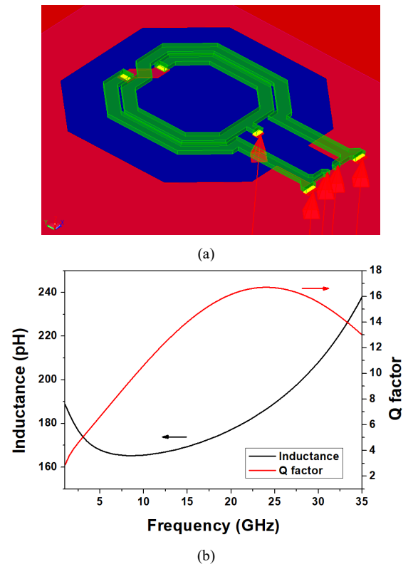
Fig. 5. (a) Structure of the spiral inductor (b) Simulated performance of the inductor.
