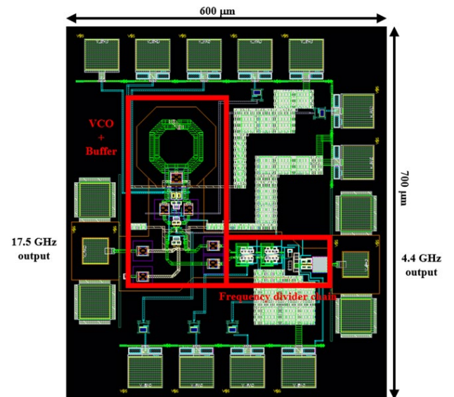
Fig. 15. Layout of the VCO integrated with the frequency divider chain
