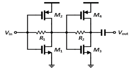
Fig. 14. Schematic of the 50-Ω driver.
