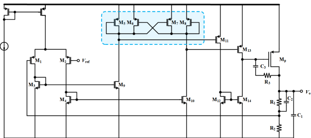
Fig. 4. Previous schematic of a capacitor-less LDO regulator
