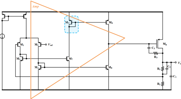
Fig. 3. Original schematic of a capacitor-less LDO regulator
