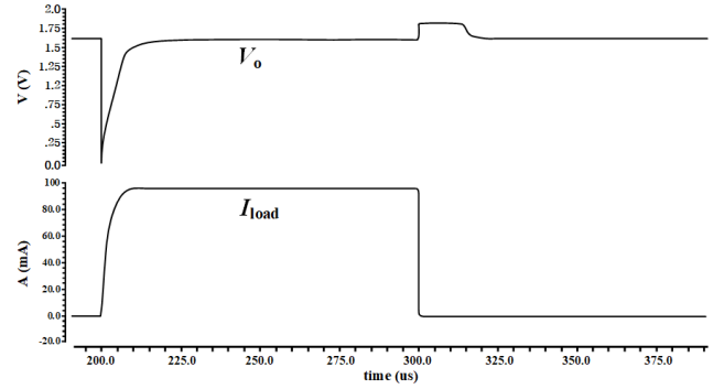
Fig. 5. Simulation of a previous schematic LDO regulator
