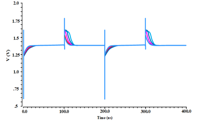
Fig. 15. Proposed LDO line transient
