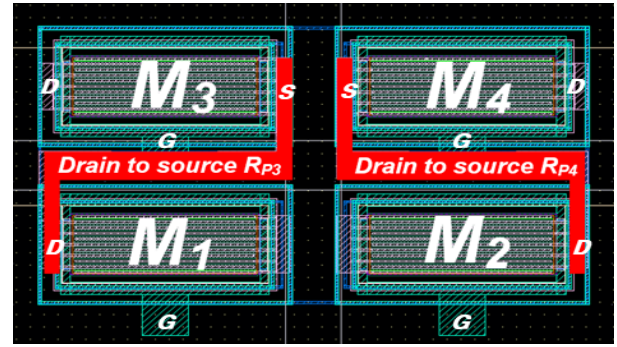
Fig. 9. Drain to source layout
