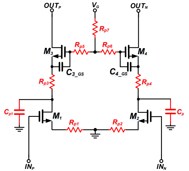
Fig. 5. Parasitic elements in drive stage of PA
