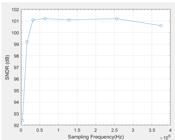
Fig.12. SNDR versus f_s from 37.5 kHz to 3.75 MHz.
