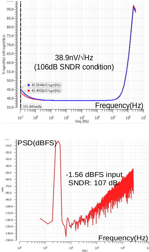
Fig. 5. PNOISE result of the first integrator and SNDR of the designed ADC which only loop-filter's noise is activated.
