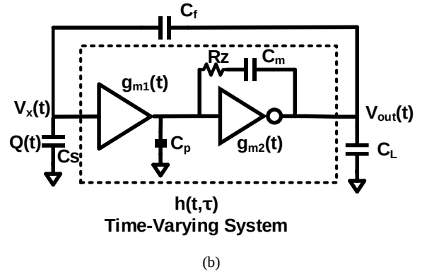
Fig. 4. (a) Proposed FIA (single-ended equivalent) and (b) SC circuit configuration.
