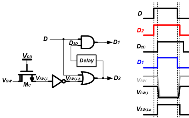
Fig. 7. Proposed adaptive dead-time generator.
