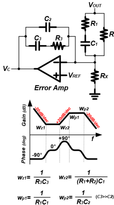
Fig. 5. Type-III compensator.
