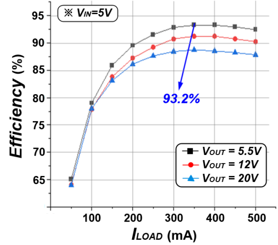
Fig. 13. Simulated efficiency with different V_{OUT} under different I_{LOAD} .
