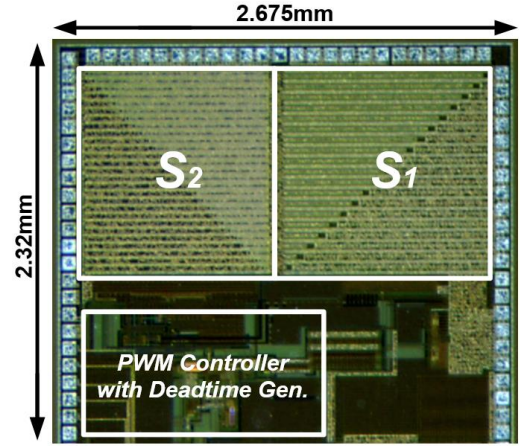
Fig. 8. Chip micrograph.
