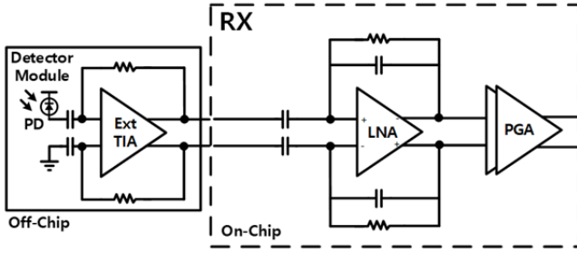
Fig. 4. Analog Front-End of FDNIRS IC
