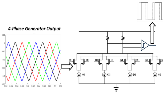
Fig. 9. Operation of phase interpolator inside the DLL block
