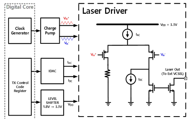
Fig. 11. FDNIRS IC TX laser driver schematic
