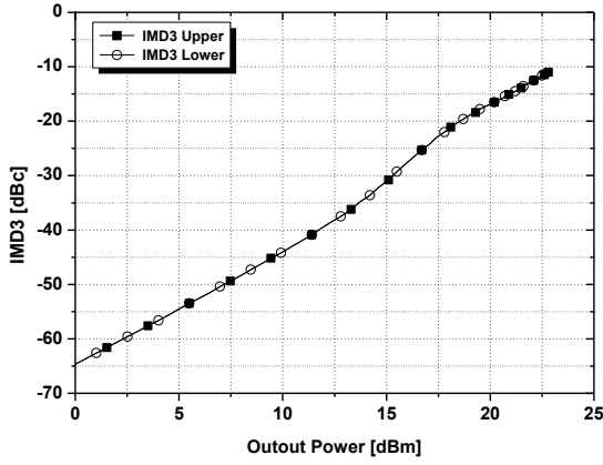
Fig. 9. Simulated IMD3
