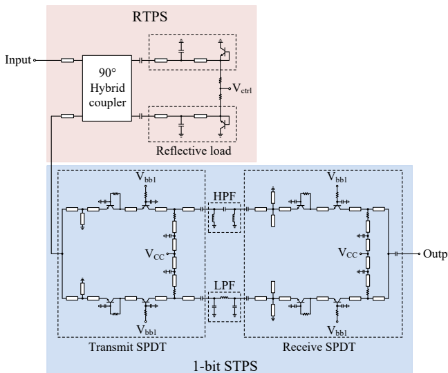
Fig. 2. Schematic of the proposed phase shifter.
