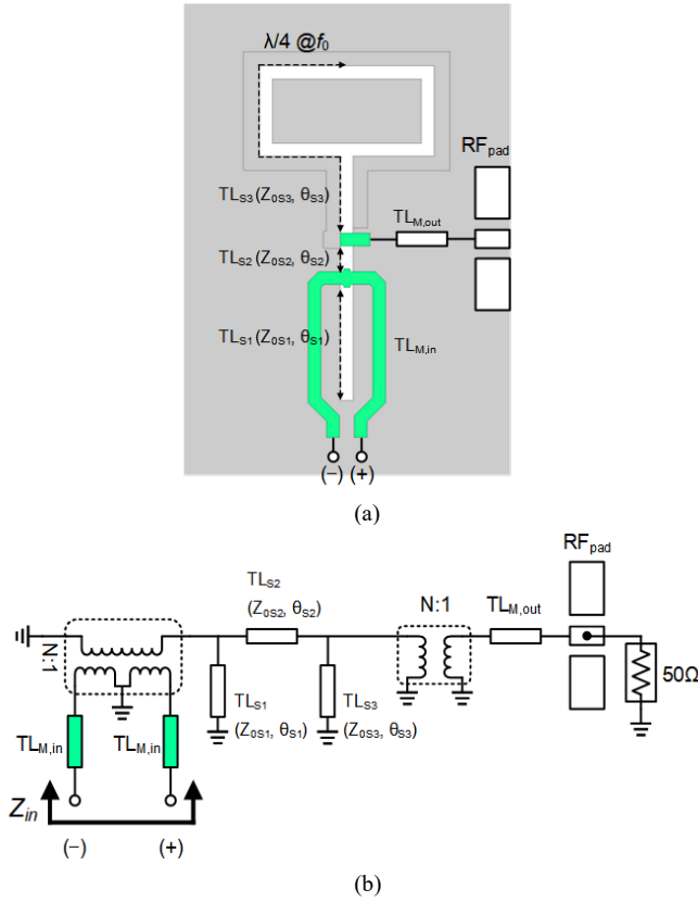
Fig. 7. (a) Top view and (b) equivalent circuit of the slotline power combiner.
