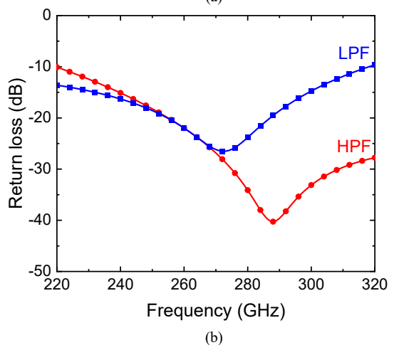
Fig. 3. Simulated (a) amplitude and phase difference and (b) return loss of the low-pass filter and high-pass filter.
