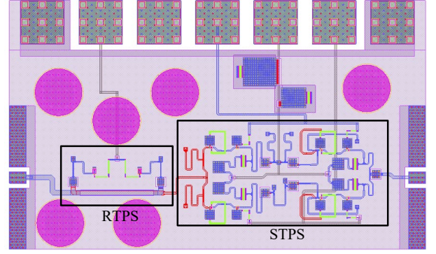
Fig. 9. Layout of the phase shifter.
