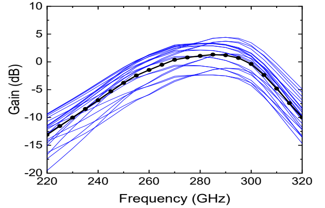
Fig. 10. Simulated gain performance of the phase shifter.
