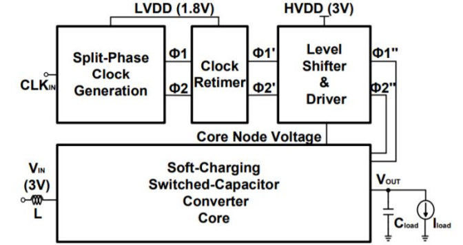
Fig. 10. Block diagram of soft-charging Cockcroft-Walton SC converter
