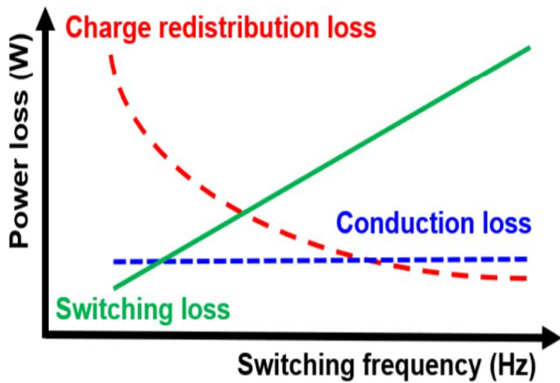
Fig. 2. Power losses of a typical SC converter
